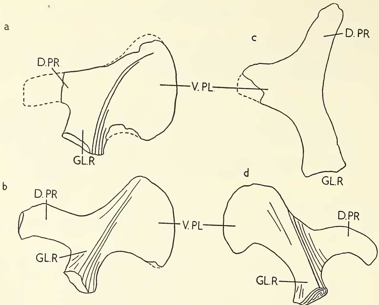
TEXT-FIG. 1. Scapulae in ventral view. a , Kronosaurus queenlandicus Longman, right scapula, Lower Cretaceous. Mus. Comp. Zool. Harvard 1285. Figured by White 1940, fig. 11a. \times \frac{1}{13} . b , Pliosaurus sp., right scapula, Kimeridgian. B.M. (N.H.) R. 287. Listed by Lydekker 1889, p. 126. \times \frac{1}{10} . c , Pliosaurus macromeris Phillips, left scapula, Kimeridgian. Sedgk. Mus. J. 35990. \times \frac{1}{8} . d , Peloneustes philarchus (Seeley), left scapula, Oxfordian. B.M. (N.H.) R. 3318. Figured by Andrews 1913, fig. 21. \times \frac{1}{5} . D. PR., dorsal process; GL. R., glenoid ramus; V. PL., ventral plate.
